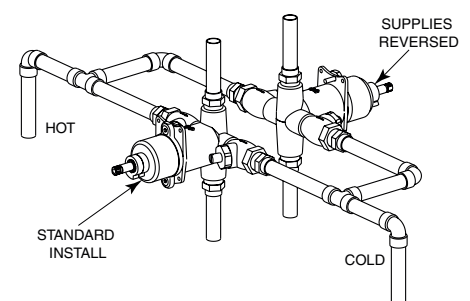
"Back-to-Back" Installation
