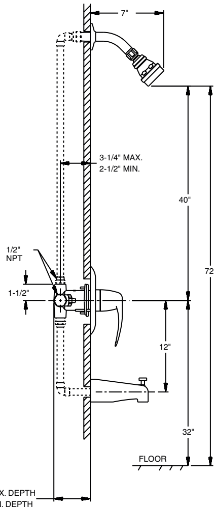
Tub/Shower Installation
