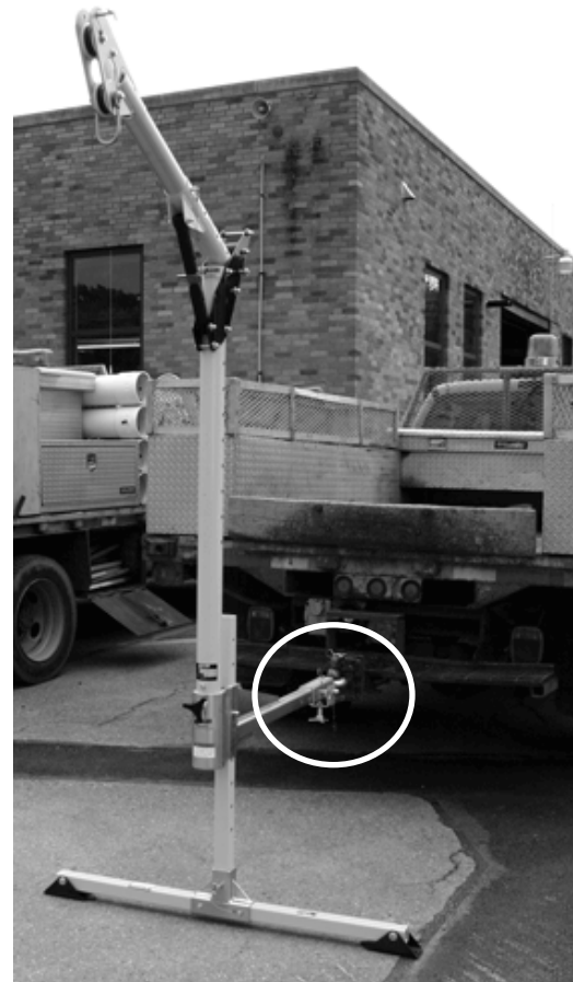
Pintle Hitch Adapter installed between the DH-12 and vehicle.
