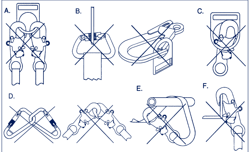
Figure 3 - Raccordements inappropriés
