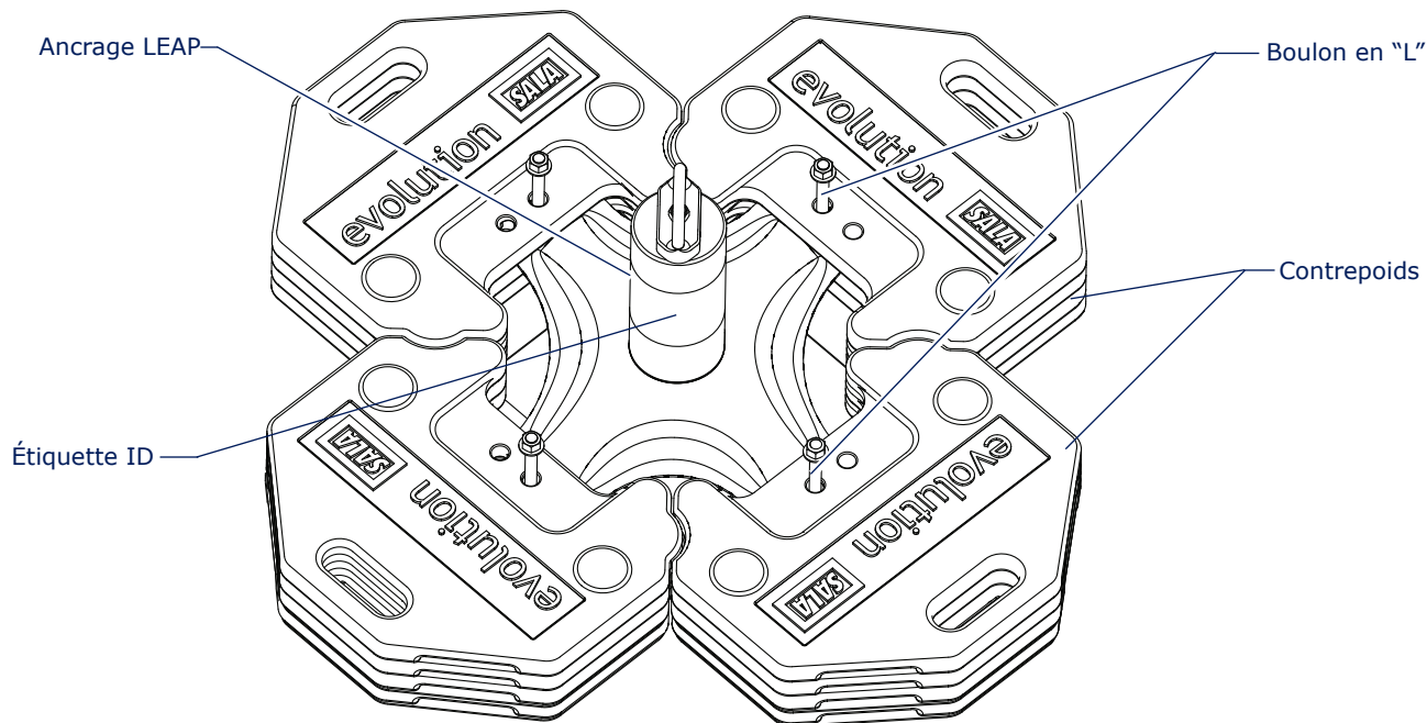
Figure 1 - Evolution Counterweight System assemblé
