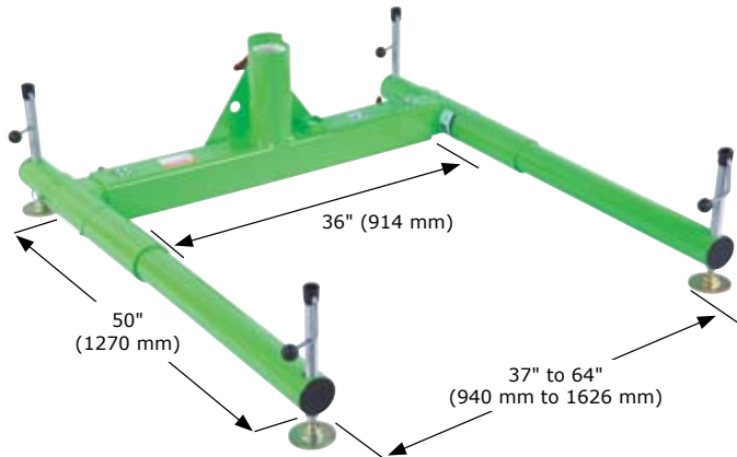
Advanced 3-Piece Expandable Base For Max. 29" (737 mm) Offset
