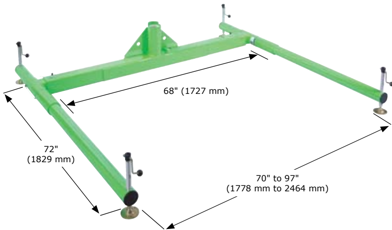
Advanced 3-Piece Expandable Base For Max. 48" (1219 mm) Offset
