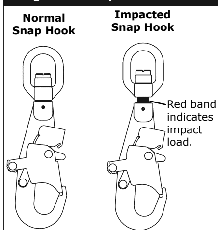
Figure 7 - Impact Indicator
